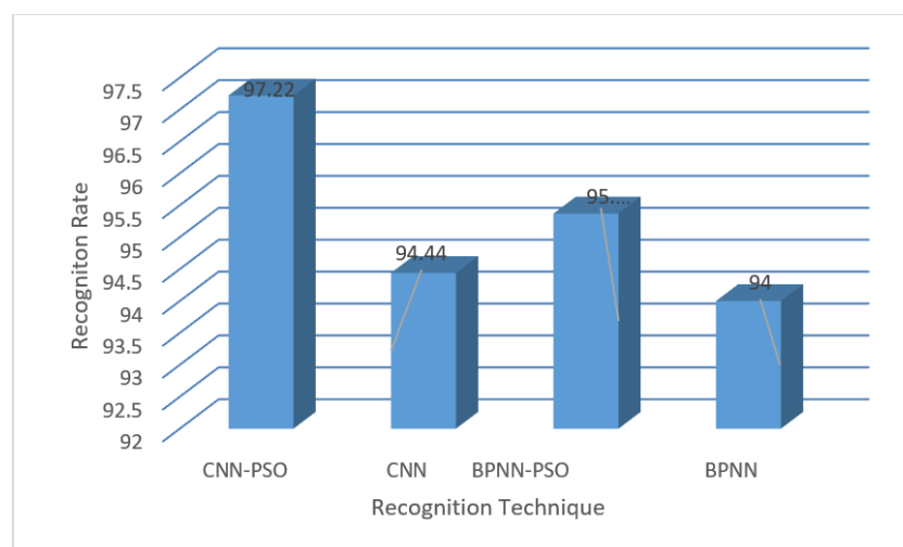
Figure A2: Recognition Rate of CASIA
