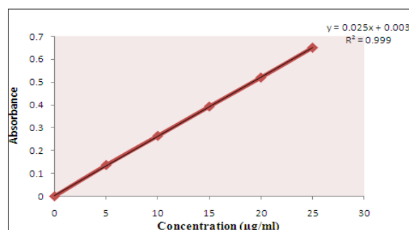
Fig. 1 Calibration curve of lovastatin in 0.1 HCL at 228nm
