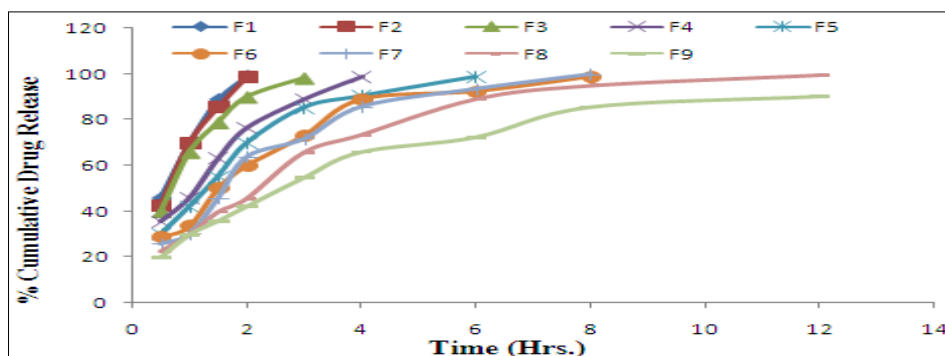
Fig.3 In-vitro drug release study of GRF tablets
