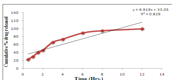
Fig. 4 Zero order release Kinetics
