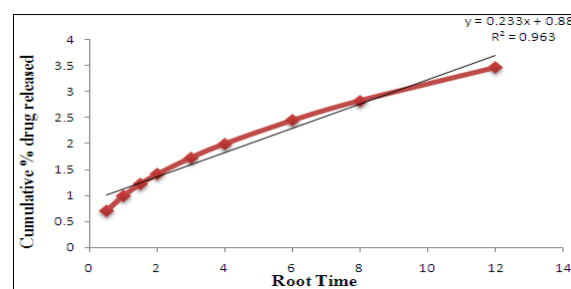
Fig. 6 Higuchi release Kinetics
