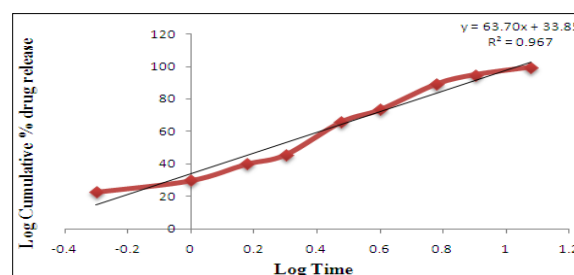
Fig. 7 Korsmeyer-Peppas release Kinetics
