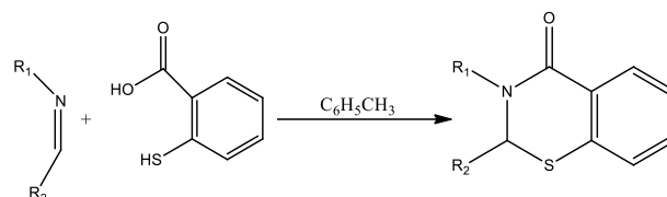
Scheme 1: Reaction scheme for synthesizing 1,3-benzothiazine-4-one derivatives
